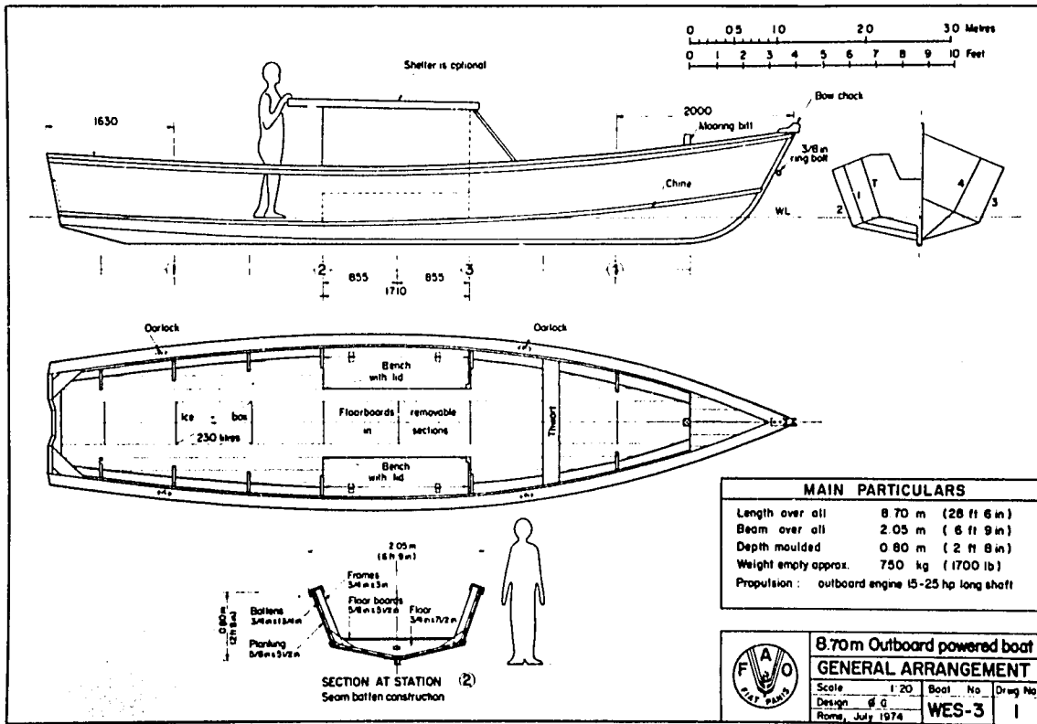
Fig. 1. A 28-ft outboard powered boat suitable for village fishery operations.
