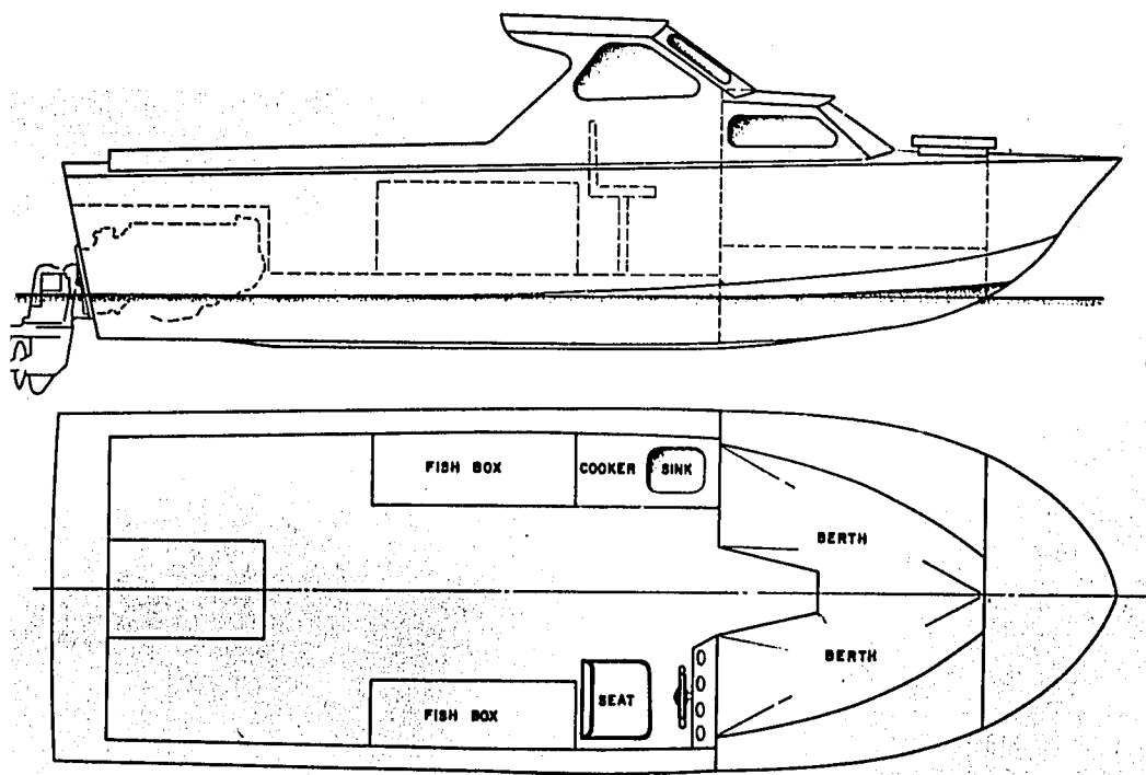
Fig. 2. Typical layout for a modified 27-ft stock hull.
