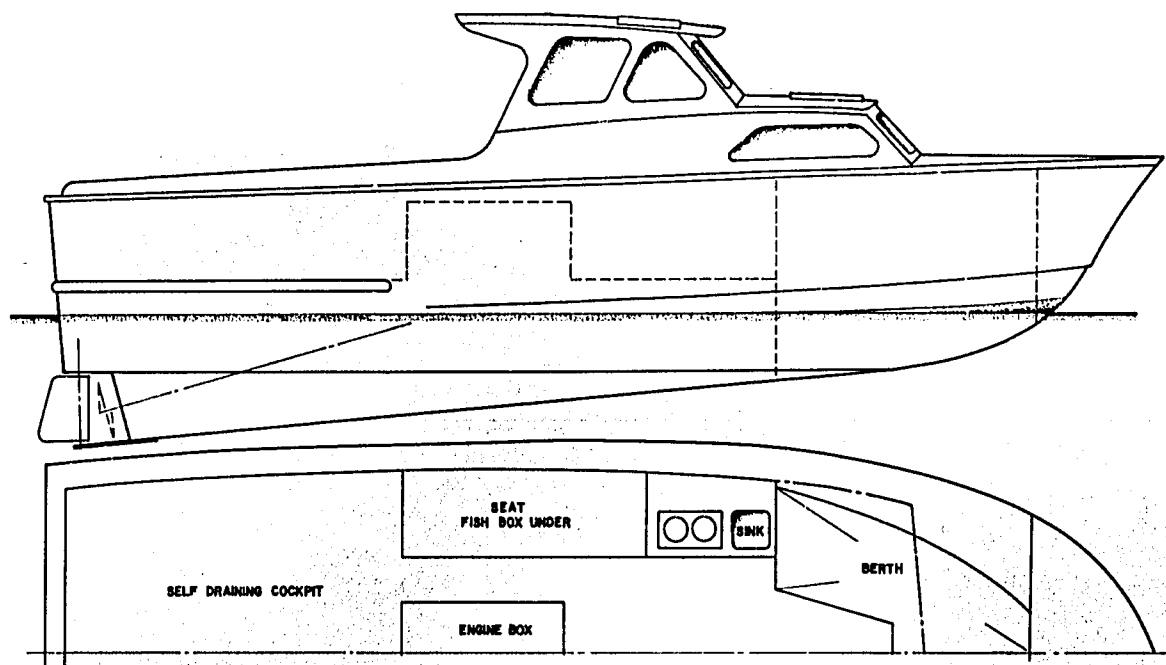
Fig. 3. Layout for a modified 27-ft stock hull used to build boats which were shipped to Fiji.
